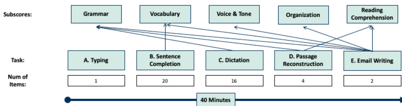
Figure 1. Relation of subscores to item types
